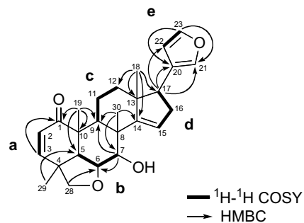
Figure 1. Selected 2D NMR correlations for ceramicine B ( 1 ).
